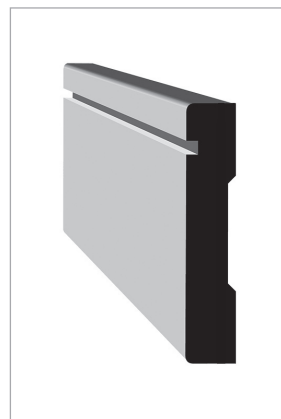
T-191A 5/8" x 3"
