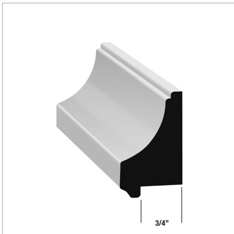
T-278 1-1/16" X 1-3/4" 16'
