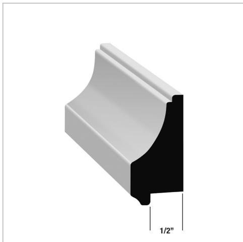
T-277 7/8" X 1-1/4" 16'
